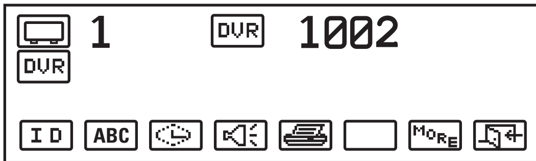
Figure 49. DVR Menu 3
